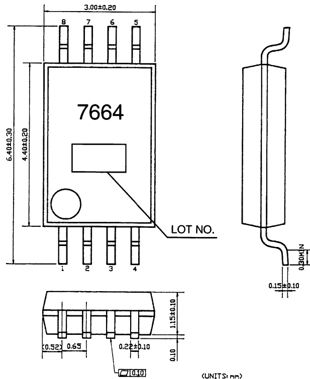
Figure 1 SSOPB 8PIN (Plastic Mold)
