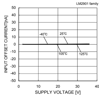
Fig. 75 Input Offset Current – Supply Voltage
