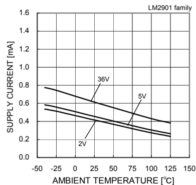
Fig. 66 Supply Current – Ambient Temperature
